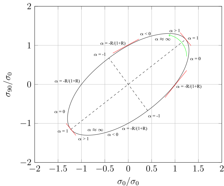
Fig. 11: Illustration of different \alpha -values on different locations of the yield surface. When the 90° occurs in the critical strain path, the element jumps on the yield locus following the green arrow.
