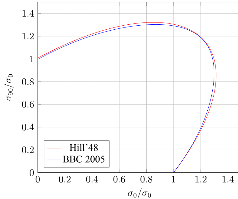
Fig. 6: Comparison of the yield loci for the VDA239 CR4 mild steel when applying a Hill'48 and BBC 2005 material model.
