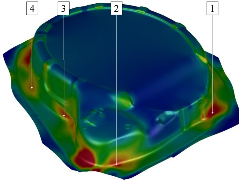
Fig. 8: Arbitrary control elements in areas with high plastic strain values.
